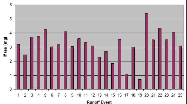
Average Nitrate Removed by Soxx System
